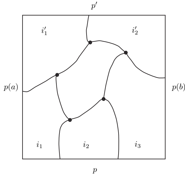
Figure 2: Proof of Theorem 3.4, part ii)
