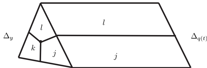
Figure 12: Labelled partition for the proof of G3)
