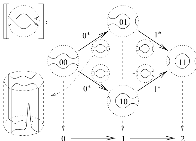
Figure 1: The Khovanov complex of a 2-crossing tangle
