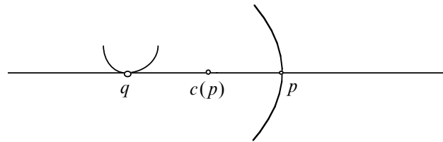
(p, q) is a type 1 normal-tangent pair
