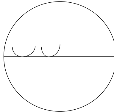
Type 2 double supporting geodesic
