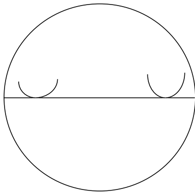
Type 1 double supporting geodesic
