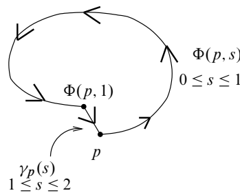
Figure 5: The map f: S^1 \rightarrow M
