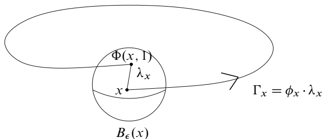
Figure 1: closed up flowline
