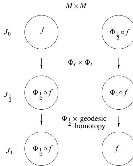
Figure 3: The homotopy J
