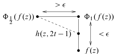
Figure 4: J_t does not intersect \Delta
