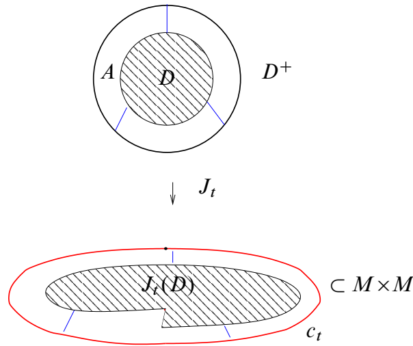
Figure 6: Extending J
