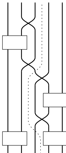
Figure 4: Possible braid shadow for a braid satisfying b_5(K) = 8 . The dotted line points out that the closed braid will be a connected sum.
