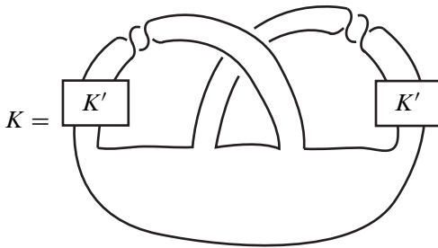
Figure 12: Order 2 in algebraic concordance group
