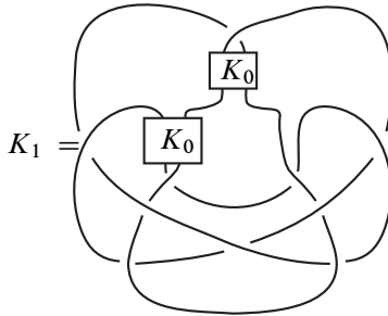
Figure 3: Algebraically slice knots K_1
