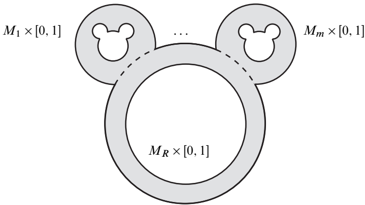
Figure 9: The cobordism E
