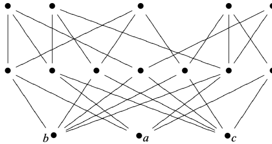
Figure 5: A homotopically trivial non-collapsible space of 15 points.
