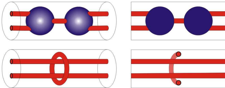
Figure 14: The homeomorphism corresponding to the 1-unzip
