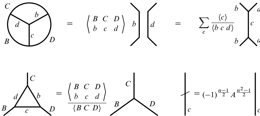
Figure 8: The value of the skein of the labeled standard tetrahedron is the six- j symbol defined below. The fusion formula reverses the unzip move, the half twist formula undoes the half twist move and the triangle formula undoes the triangle move.
