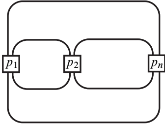
Figure 2: A general pretzel link P(p_1, \dots, p_n)
