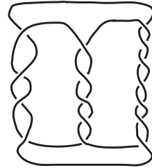
Figure 3: The (-3, 5, 7) pretzel knot
