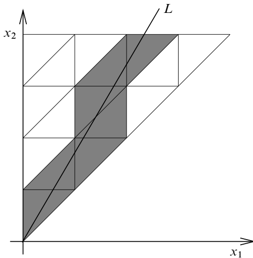
Figure 4: Illustrating the construction of the disc D of Lemma 6.1 in the case n = 2, \ell = 4 . A line L with irrational slope \alpha > 1 meets each line defining the triangulation exactly once, and except at \mathbf{0} never passes through the intersection of two such lines. We take D to be the union of the 2-simplices intersecting L (shaded grey). The disc D contains at least \ell n -simplices (here at least 4), since it must include at least one from each horizontal slice.
