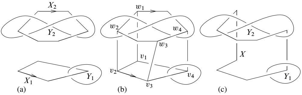
Figure 2: Illustrating the proof of Flapan’s [2, Lemma 2], the n = 1 case of our Lemma 7.2 (the four-to-three lemma for integral linking number).
