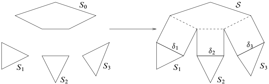
Figure 3: Illustrating Lemma 2.5 in the case n = 1, k = 3 . The sphere S_0 is used to construct a sphere \mathcal{S} meeting S_i in a single n -simplex \delta_i for i = 1, 2, 3 .
