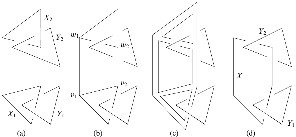
Figure 1: Illustrating the proof of Lemma 3.1 (the four-to-three lemma for mod two linking number) in the case n = 1 .
