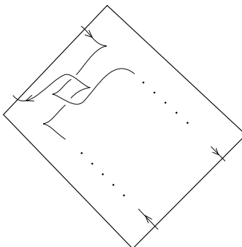
Figure 3: The module with n full left twists provides knots K_2(n) with vanishing Thurston–Bennequin numbers. In the diagram the module is already in Legendrian position. Obviously, by adding a left and a right cusp to the diagram we get a Legendrian unknot with Thurston–Bennequin number -1 .
