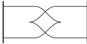
Figure 3: The Legendrian submanifold of J^1 S^1 represented by this front diagram has a linear-at-infinity generating family, but is not horizontally displaceable.
