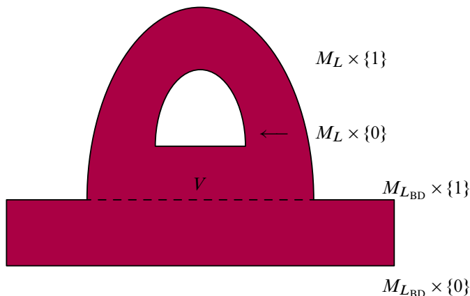
Figure 11: The space X
