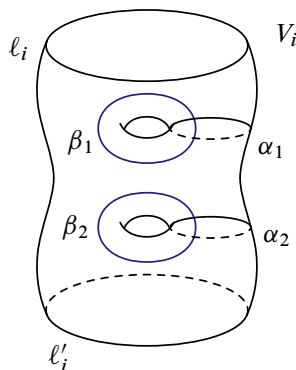
Figure 16: The first stage grope, V_i , with symplectic basis \{\alpha_i, \beta_i\}_{i=1,2}
