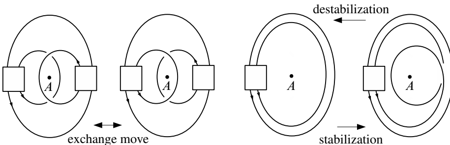
Figure 1: On the left, an exchange move; on the right, stabilization (destabilization)
