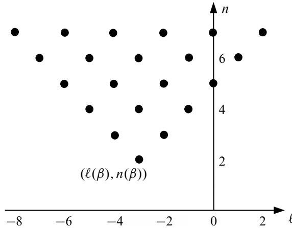
Figure 11: The cone of a braid \beta in the (\ell, n) -plane
