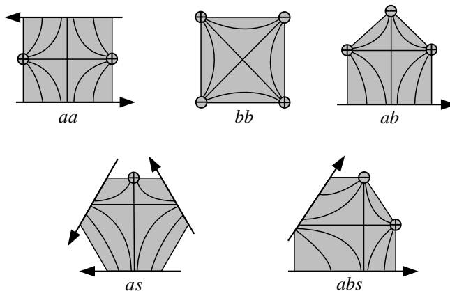
Figure 2: The five types of saddle singularities, classified by the types of nonsingular arcs interacting to form the singularity. The parities of the vertices may be reversed provided the orientations of the transverse boundary arcs are compatibly reversed.
