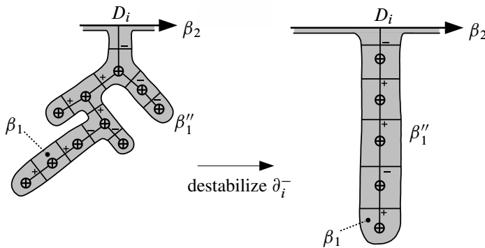
Figure 7: On the left, D_i , whose vertex-singularity graph is a tree after stabilizing \partial_i^- ; on the right, D_i , whose graph is a linear tree after destabilizing \partial_i^-
