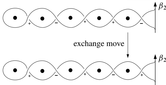
Figure 8: An exchange move involving the two consecutive singularities closest to the \beta_2 -end of the D_i linear tree. The black dots represent intersections of the braid axis A with D_i .
