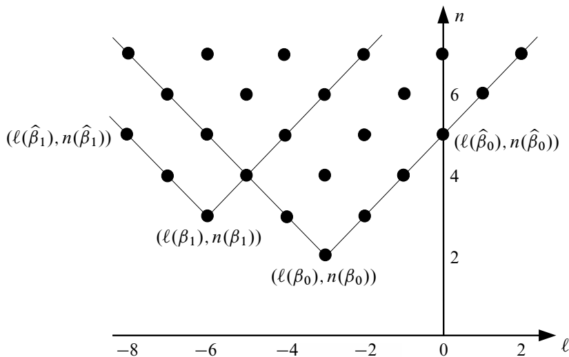
Figure 12: Two cones with neither one contained in the other
