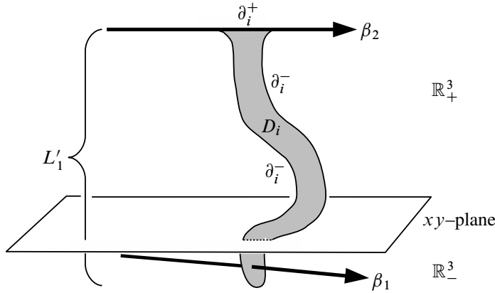
Figure 5: The link L'_1 and discs D_i after isotoping \beta'_2 to \beta_2 in \mathbb{R}^3_+
