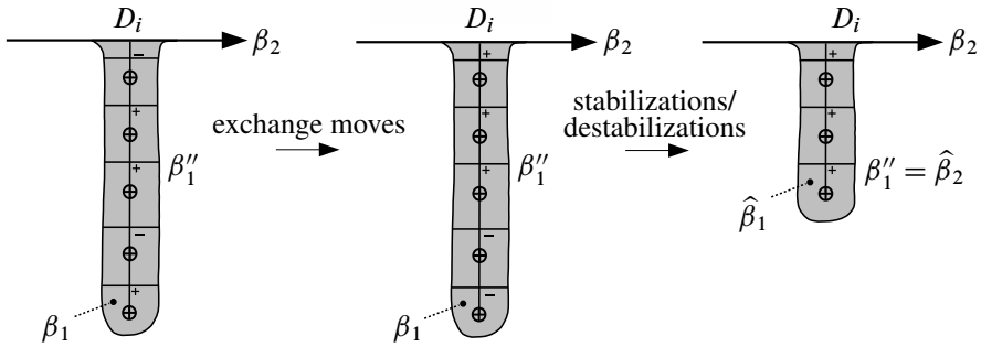
Figure 9: On the left, reordering of singularities using exchange moves so that all positive singularities are stacked near the \beta_2 -end of D_i and all negative singularities are stacked near the \beta_1 -end. On the right, negative destabilizations of \partial_i^- , along with the corresponding negative stabilizations of \beta_1 which yield \hat{\beta}_1 , and the subsequent positive stabilizations of \beta_2 which yield \hat{\beta}_2 .
