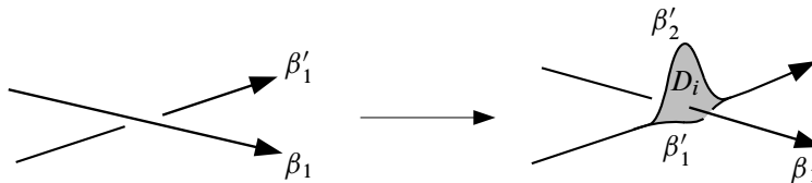
Figure 4: An under-crossing of \beta'_1 passes through \beta_1 to produce \beta'_2 , and produces a bigon disc D_i which is intersected once by \beta_1 .
