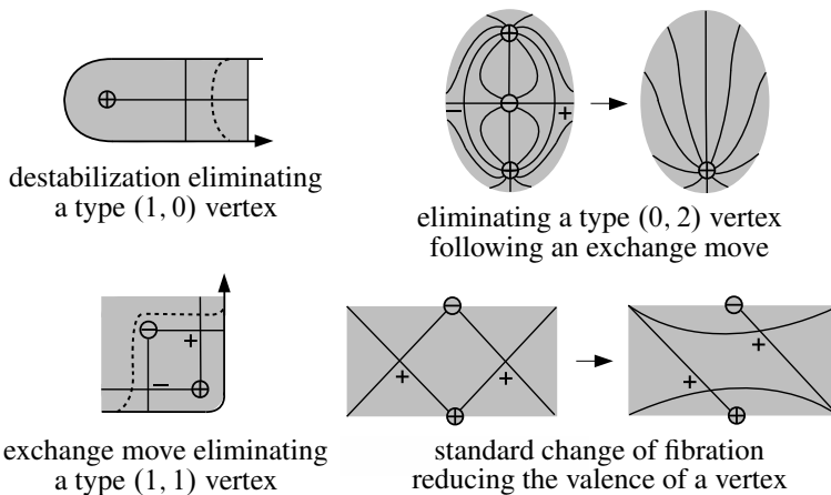
Figure 3: Eliminating, and reducing the valence of, vertices using destabilization, exchange moves and braid isotopy. In the figures on the left, the braided boundary is indicated by the bold black arrow, and the subdisc cobounded by it and the dashed line is eliminated following destabilization and an exchange move, respectively.
