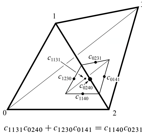
Figure 10: Ptolemy relation for the subsimplex s = 0130
