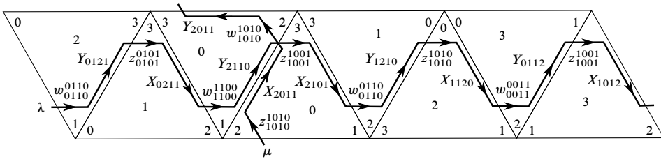
Figure 22: Generators of the peripheral fundamental group of the figure-eight knot complement. The indicated coordinates are those involved in the cusp equations at level l = 2 for n = 4 .
