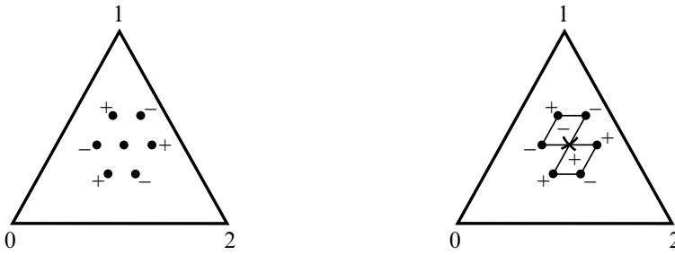
Figure 18: Left: exponents of the Ptolemy coordinates involved in the X -coordinate at t . Right: an X -coordinate as a quotient of two diamond coordinates.
