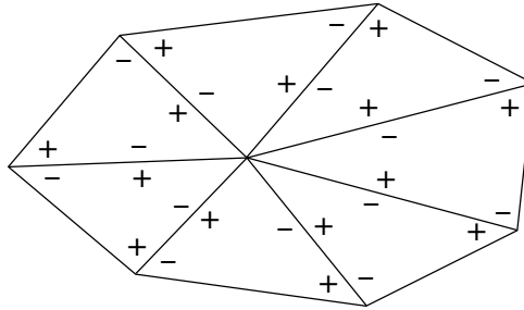
Figure 14: Cancellation of terms in \beta^* \circ \beta(p) for an edge point p
