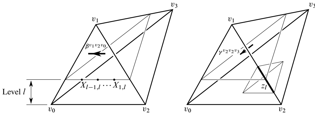
Figure 21: The terms in the simplified cusp equations at level l
