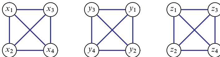
Figure 9: A graph representing \pi_1(T^4 \# T^4 \# T^4)
