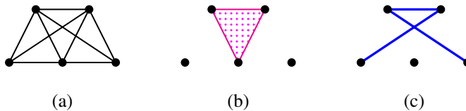
Figure 23: (a) The edges eventually created by a 4-reduction of type [a, b, c, de] , (b) the triangle created by a, b and c , and (c) the edges belonging to the maximal isotropic subspace
