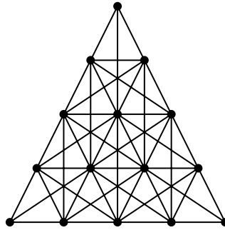
Figure 16: A graph in the hex family
