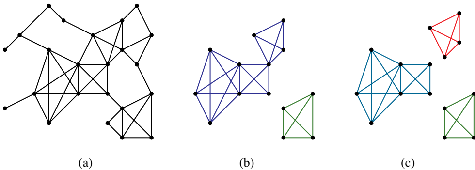
Figure 5: An example of the breakdown of a graph into disjoint subgraphs, for the calculation of h according to Theorems 1.4 and 1.5
