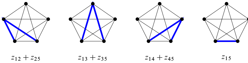
Figure 28: 4 basis elements in the radical for k = 1 and \alpha = s_{1234} + s_{2345}
