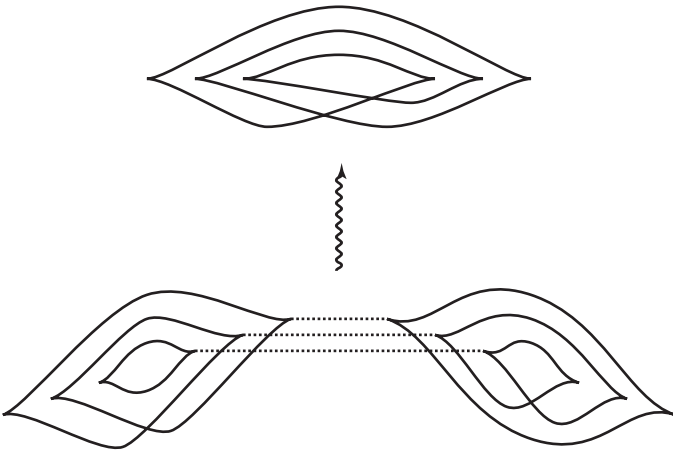
Figure 7: The construction of a Lagrangian null-cobordism of genus 0 for the zero closure of the positive braid \sigma_2\sigma_1 . The 1–handles are attached in succession from the outermost to innermost cusps.
