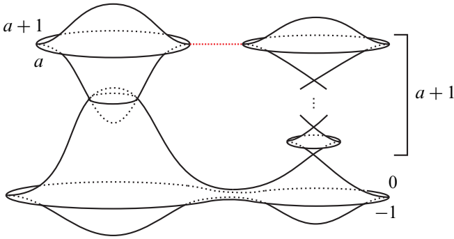
Figure 11: A scheme to construct a Legendrian sphere with \Gamma_{f_a}(t) = t^n + t^a + t^{n-1}t^{-a} with a \geq \lfloor (n-1)/2 \rfloor .
