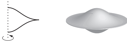
Figure 1: Spinning half of a Legendrian unknot yields a “flying saucer”
