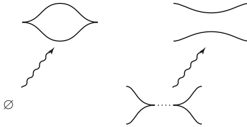
Figure 5: The modifications to the front of a 1–dimensional Legendrian that arise from attaching a 0–handle and a 1–handle
