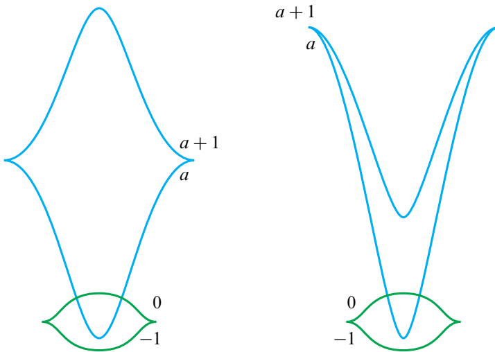
Figure 9: Two Legendrian Hopf links used in the proof of Lemma 6.8. Both have six Reeb chords along the central axis, with the length of the Reeb chord from the bottom of the upper component to the top of the lower component shorter than then Reeb chord between the bottoms of the two components.
