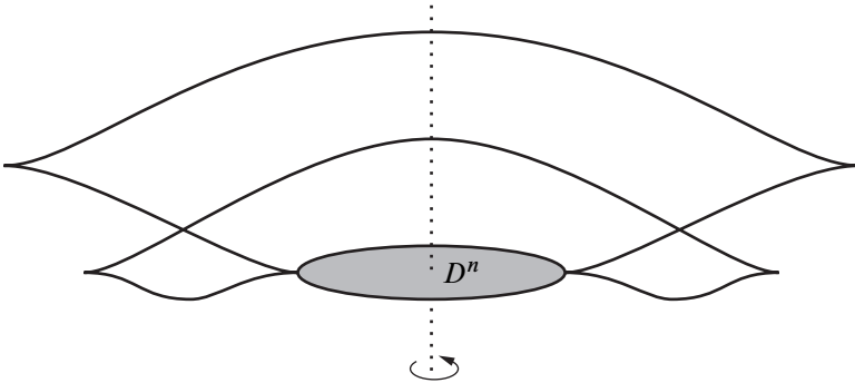
Figure 8: Spinning this unknot results in an n -dimensional Legendrian submanifold isotopic to the standard flying saucer, but having an S^{n-1} family of cusps that bounds a disk D^n on the outside.
