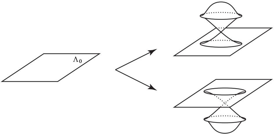
Figure 10: The higher-dimensional first Reidemeister moves
