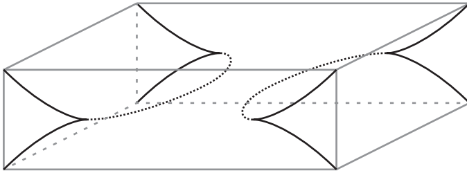
Figure 2: A schematic picture of the domain of an attaching region \sigma: D^q(1 + \lambda) \times D^{n-q}(\lambda) \times D^1(\lambda) \rightarrow M^n \times \mathbb{R} , with the preimage of the Legendrian \Lambda and the cusps \Lambda^\succ shown in solid and dotted curves respectively.
