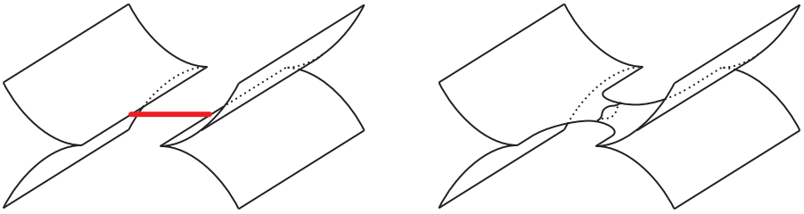
Figure 3: (a) The core disk for a 0 surgery and (b) the result of embedded surgery along the core disk for a Legendrian surface in \mathbb{R}^5 = J^1\mathbb{R}^2
