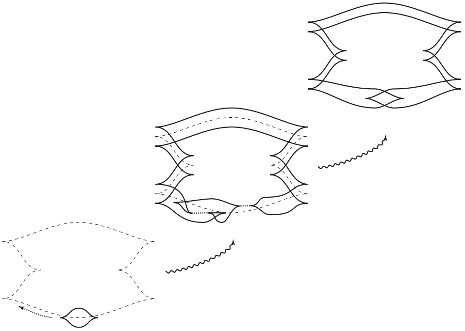
Figure 6: The construction of a Lagrangian null-cobordism for a Whitehead double
