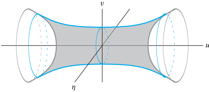
Figure 4: The handle H in the domain of f_- , with \pi_x(H) shown in grey
