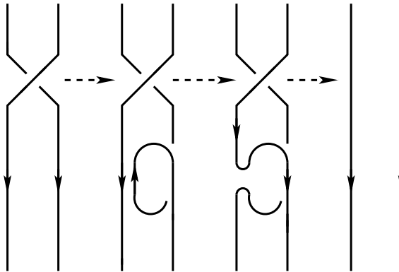
Figure 3.2: Local moves
