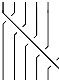
Figure 3.4: The braid \Delta for m = 6
