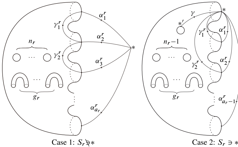
Figure 2: S_r and paths to choose generators of F' in Step 3.
