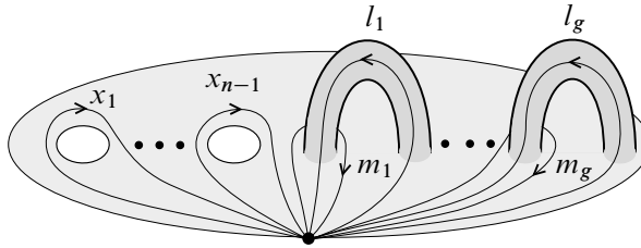
Figure 1: A generating set for \pi_1(\Sigma_{g,n}) .
