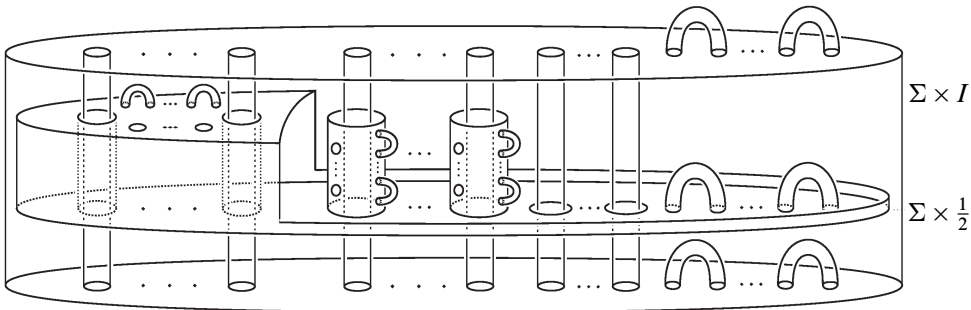
Figure 3: J(\Sigma') in \Sigma \times I .
