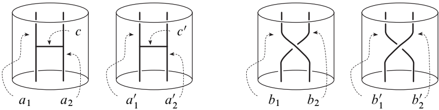
Figure 5: The arcs \mathbf{a}, \mathbf{a}', \mathbf{b}, \mathbf{b}', c, c' \subset (D \times S^1) \sqcup (D' \times S^1) (top and bottom are identified)
