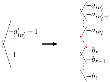
Figure 10: Finding an embedding of L .
