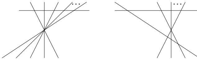
Figure 6: Symplectic line arrangements.
