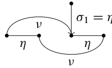
Figure 1: C\eta \wedge Cv shown horizontally, with 0-cell on the left. The element \sigma_1 is given by the map \eta on the 4-cell defined by a nullhomotopy of \eta v = 0 \in \pi_4(S^0) , as indicated in (3-1).
