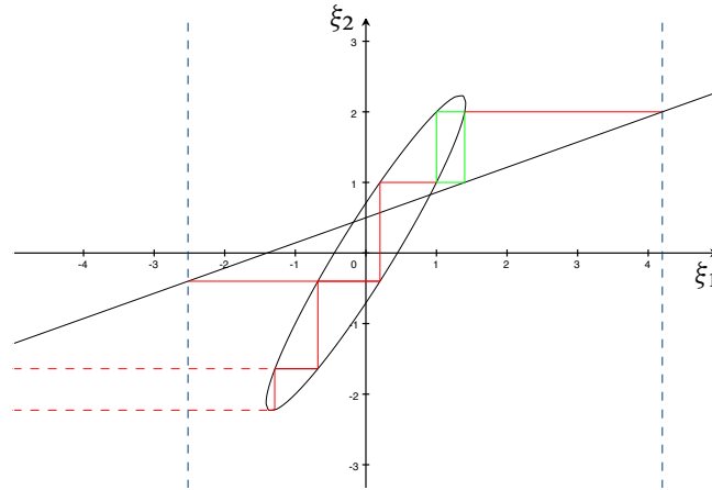
Figure 5. Section of the characteristic variety and the phase generation for corner problem (16).
