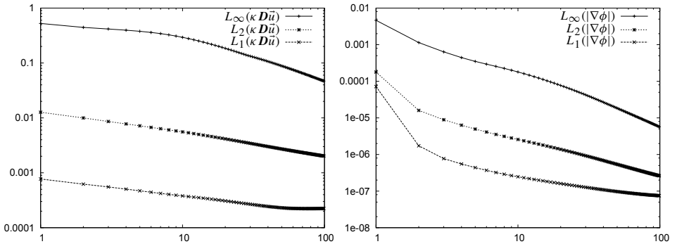
Figure 4. Norms ( L_\infty , L_2 and L_1 ) of \kappa \mathbf{D} \vec{u} (left) and \nabla \phi (right) versus the number of projection iterations in the 2D test with h = \frac{1}{256} .
