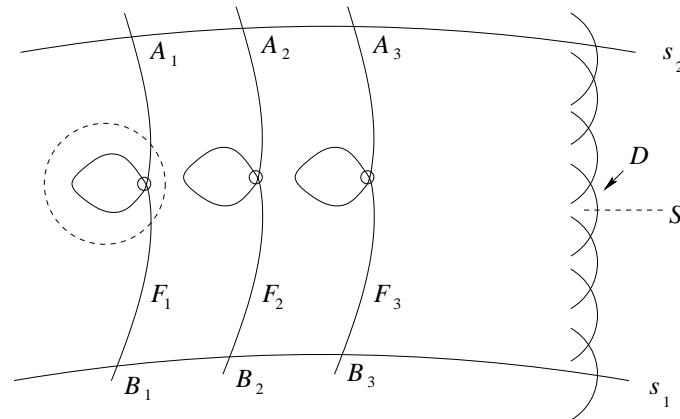
Figure 2: Singular fibers in the fibration
