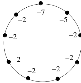
Figure 5: “Necklace” of spheres in \mathbb{C}P^2 \# 14\overline{\mathbb{C}P^2}
