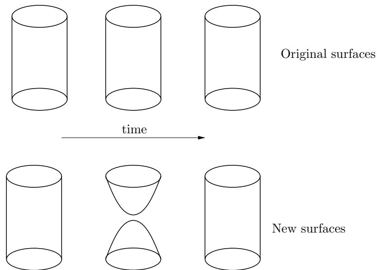
Figure 1: Pinching off a family of annuli
