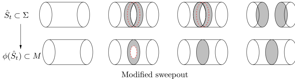
Figure 5: Doing a cut move in I_a
