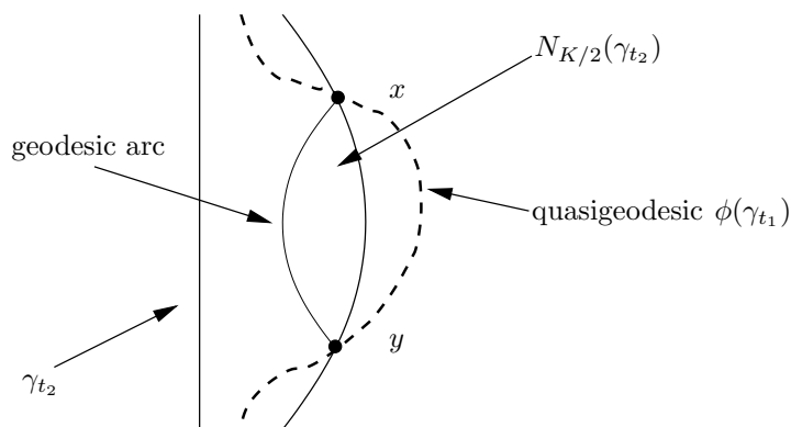
Figure 2: A K/2 -neighbourhood of a geodesic
