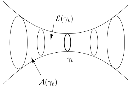
Figure 3: Annular and surgery neighbourhoods
