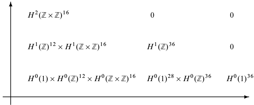
Figure 2: The E_1 page of the equivariant spectral sequence for the action \text{OP}\Sigma_4 \curvearrowright \text{MM}_4
