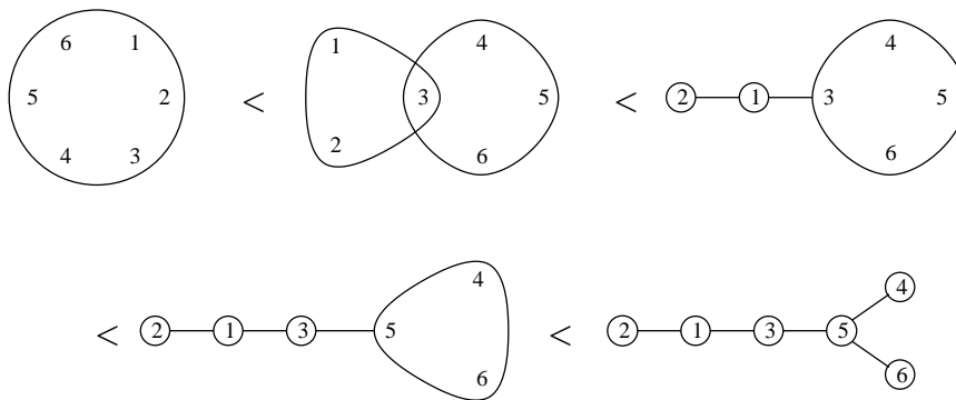
Figure 1: A maximal chain in HT_6
