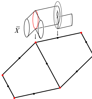
Figure 1: Constructing the exploded torus space
