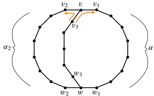
Figure 10: One of the paths of length 2 running through v must be stalling.
