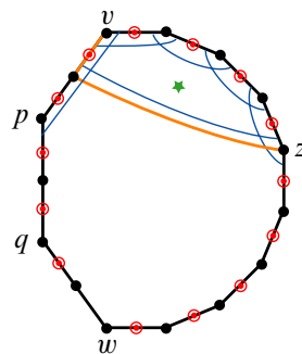
Figure 9: A 1-cut yielding a 2-cut for \alpha
