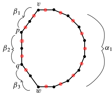
Figure 8: A dual disk diagram for a stalling cut
