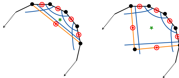
Figure 7: 1-cuts and 2-cuts arising from shells
