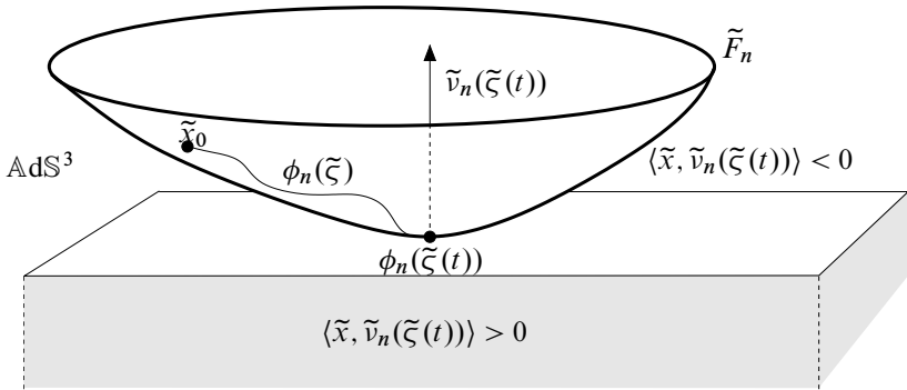
Figure 2: The product \langle \tilde{x}_0, \tilde{v}_n(\zeta(t)) \rangle is negative.
