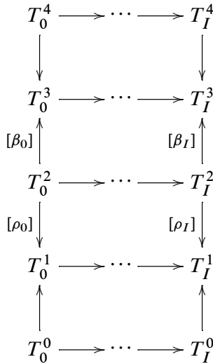
Figure 13: Each of the four horizontal rectangles is a combing rectangle. We assume that every column is a normalized W zig-zag and that the tree T_I^2 has an edge e containing both red and blue edgelets.
