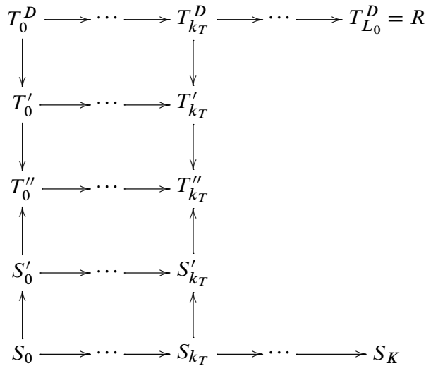
Figure 22: The result of a parallel simplistic pushdown on Figure 21, in the case when T_{k_T}^0 \neq \beta_{k_T} \cup \rho_{k_T} . Concatenating the upper two combing rectangles into a single one, and the same for the lower two, we obtain a projection diagram.
