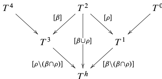
Figure 7: A simplistic pushdown works if \beta \cup \rho \subset T^2 is a proper subgraph.
