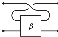
Figure 8: The string link T(\beta)
