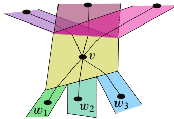
Figure 2: A section of an embedded dual digraph
