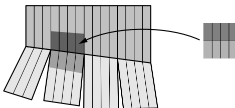
Figure 1: A hinge on a branched surface
