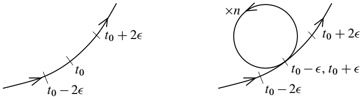
Figure 8: Curves \gamma and \gamma^{[t_0\#n]}
