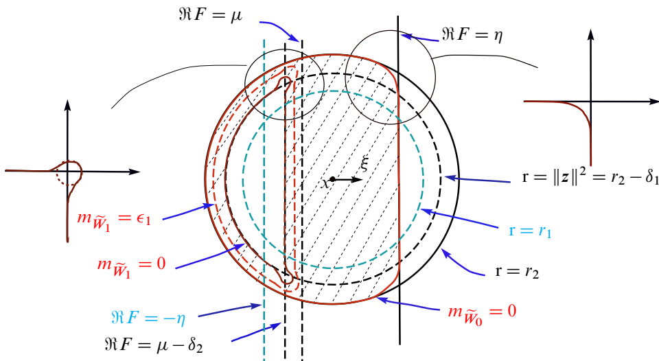
Figure 2: Construction of U : U is the shaded area, and the leftmost and rightmost pictures are illustrating the local smoothing process for the corners.
