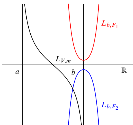
Figure 1: A picture illustrating a standard brane, two local Morse branes and their Floer cohomology for X = \mathbb{R}
