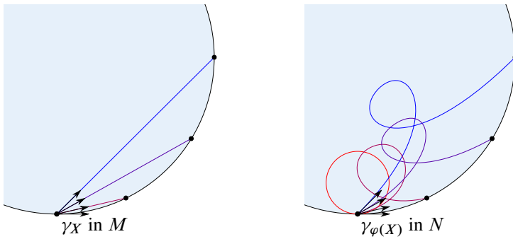
Figure 4: Closed geodesics?
