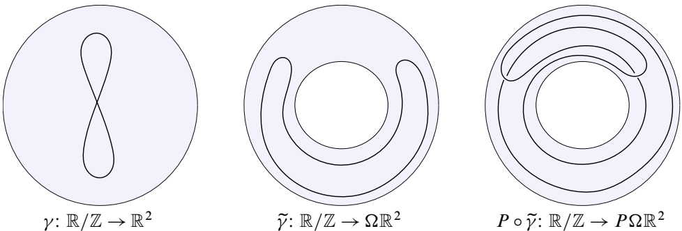
Figure 5: The unit tangent vector field of the figure-eight curve is unknotted while the projectivized unit tangent vector field of the figure-eight curve is knotted. Here the solid tori ( \Omega\mathbb{R}^2 and P\Omega\mathbb{R}^2 ) are projected to annuli for illustration.
