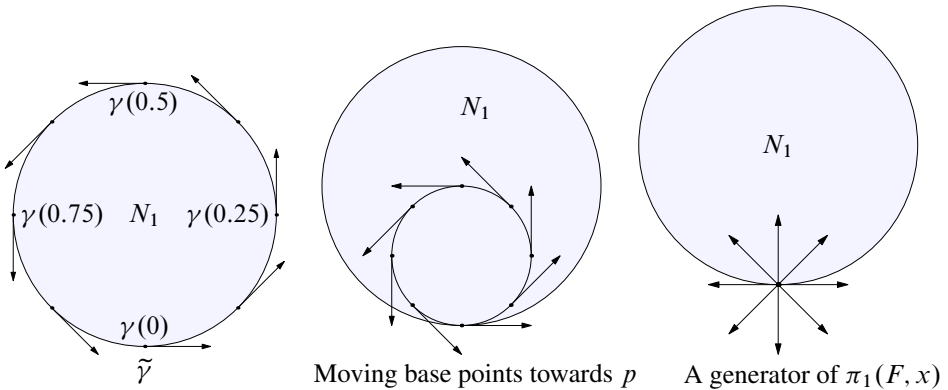
Figure 6: \tilde{\gamma} is homotopic to a generator of \pi_1(F, x)
