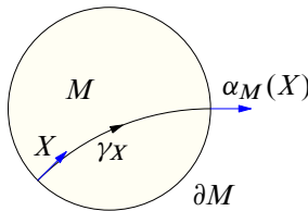
Figure 2: The scattering map \alpha_M
