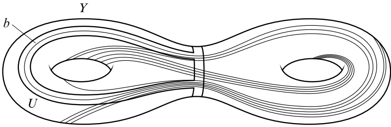
Figure 1: The \delta -neighborhood U of an arc b in \lambda \cap Y is a regular neighborhood in Y with at least one essential boundary curve. For i sufficiently large, the Hausdorff distance of \alpha_i and \lambda is less than \delta , so \alpha_i \cap Y is contained in U .
