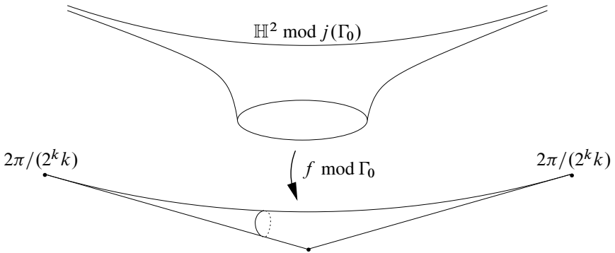
Figure 21: The representation \rho_k can be seen as the holonomy of a singular hyperbolic metric on a sphere with three cone points of angle 2\pi/(2^k k) , 2\pi/(2^k k) and close to 2\pi . The angle at the third cone point determines the distance between the other two, and is adjusted so that no equivariant map f can be better than (1-o(1)) -Lipschitz as k \rightarrow +\infty .
