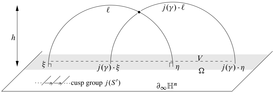
Figure 7: Two leaves \ell and j(\gamma) \cdot \ell which nearly intersect, at an angle close to \frac{\pi}{3} (in the upper half-space model of \mathbb{H}^n )
