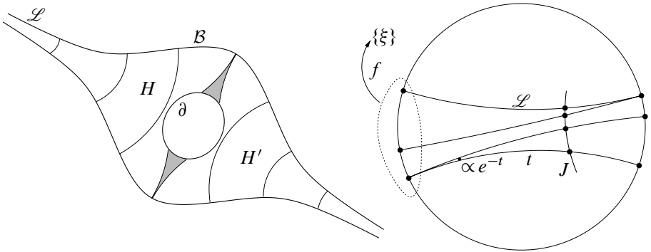
Figure 18: The one-holed bigon B bounded by the irrational lamination \mathcal{L} (left). The symbol \partial denotes the boundary of the convex core. The function \varphi is constant on the shaded area; elsewhere its level curves are pieces of horocycles. Right, the Lipschitz map f must collapse all lines of \mathcal{L} if C < 1 , because e^{-Ct} \gg e^{-t} for large t .
