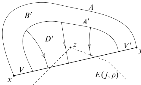
Figure 15: Improving the local Lipschitz constant at z
