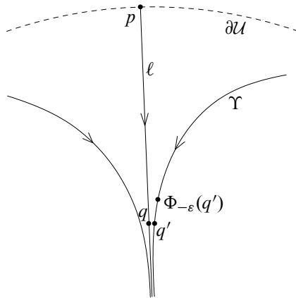
Figure 12: Flowing back by \Phi_{-\epsilon} brings q' closer to p .
