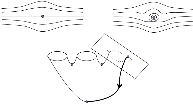
Figure 1: Top left: level sets of a Morse–Smale function for a neighborhood of an unperturbed III d boundary, viewed as a puncture. Top right: level sets of the perturbed Morse–Smale function. Note that the central disk, which rotates under the Hamiltonian flow, is excised to glue with other components. Bottom: the plane represents part of the pseudo-Anosov with type III d boundary. The remainder of the surface represents a component with type Ia fixed points. The unique flow-line is shown in bold.
