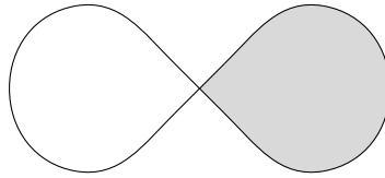
Figure 10: Computation of \mathfrak{t} for the Legendrian unknot. The disk drawn lies in an (n-1) -dimensional family that sweeps the filling once.
