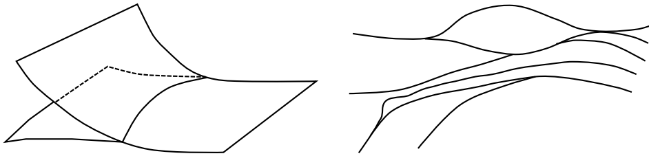
Figure 1: The branching of center and center stable leaves. Left: two center stable leaves sharing a region. Right: distinct center leaves inside a center stable leaf.
