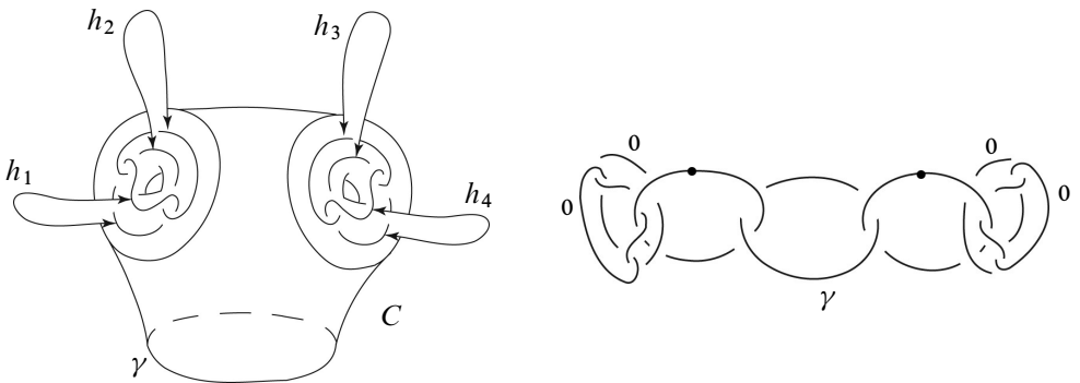
Figure 2: The handlebody C (a Bing cell of height 1): a schematic picture and a Kirby diagram
