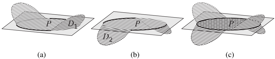
Figure 1: (a) A 2-disk D_1 \subset F_1 \subset \mathbb{R}^2 \times [0, \infty[ intersects \mathbb{R}^2 \times \{0\} in the round 2-disk P . (b) A similar 2-disk D_2 \subset F_2 \subset \mathbb{R}^2 \times ]-\infty, 0] . (c) D_1 \cup D_2 is a 2-disk on F = F_1 *_P F_2 \subset \mathbb{R}^3 .
