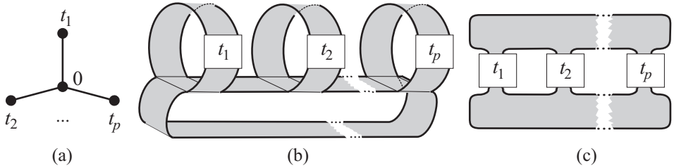
Figure 8: (a) \text{star}(0; t_1, t_2, \dots, t_p) . (b) Star surface \text{sp}(\text{star}(0; t_1, t_2, \dots, t_p)) . (c) Pretzel surface \mathcal{P}(t_1, \dots, t_p) .
