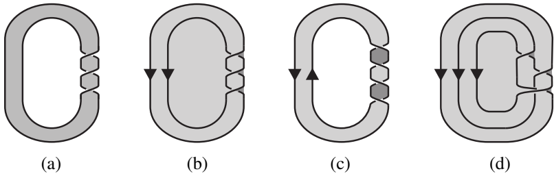
Figure 5: (a) The unoriented unknotted strip \mathcal{S}(\mathbb{O}, 3) with 3 half-twists, and its unoriented boundary. (b) For t > 0 , \partial\mathcal{S}(\mathbb{O}, t)^\circ bounds the quasipositive braided Seifert surface S(\sigma_1, \dots, \sigma_t) with all b_i = \sigma_1 \in B_2 . (c) For s < 0 , \partial\mathcal{S}(\mathbb{O}, 2s)^\circ bounds the quasipositive annular Seifert surface \mathcal{A}(\mathbb{O}, s) . (d) \mathcal{A}(\mathbb{O}, -2) as the quasipositive braided Seifert surface S(\sigma_1 \sigma_2, \sigma_2, \sigma_1) .
