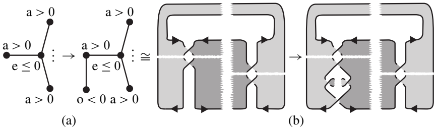
Figure 14: The illustrated strip-plumbing preserves diagrammatic positivity and therefore strong quasipositivity, but cannot be performed by plumbing quasipositive Seifert surfaces.
