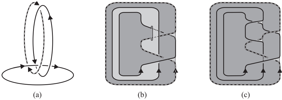
Figure 3: (a) \mathcal{H}_-(3, 2) = \mathcal{L}_\infty(z_0(z_0z_1 - 1)) . (b) \mathbb{C} -span of \mathcal{L}_\infty(z_0(z_0z_1 - 1)) in D^4(\mathbf{0}, 1/\varepsilon) , represented as a ribbon-immersed surface in S^3 . ( Figure 2(d) suggests the analogous surface for any \mathcal{H}_-(p, p-1) with p \geq 3 .) (c) The fiber surface of \mathcal{L}_\infty(z_0(z_0z_1 - 1)) .
