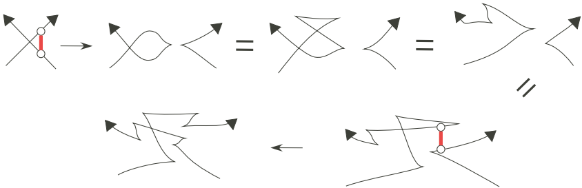
Figure 22. A sequence of two oriented surgeries in a neighborhood of a negative crossing that topologically change the crossing.
