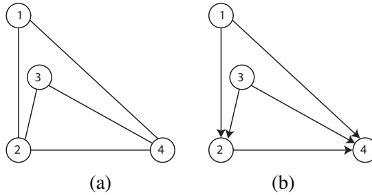
Figure 2. A hierchal orientation \vec{G}_{\mathcal{R}} having P(\vec{G}_{\mathcal{R}}) < M(\vec{G}_{\mathcal{R}}) = Z(\vec{G}_{\mathcal{R}}) .
