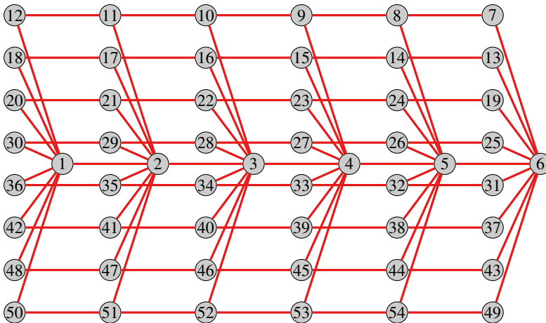
Figure 24. A prime vertex labeling of S_8 \times P_6 .
