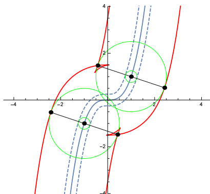
Figure 9. The envelope curves associated to the families of circles of constant radius \frac{1}{4} and 1 and centered on the curve y = t^3 . It is plausible that the dashed envelope curves have the central cubic as their midset, but this visibly cannot be the case for the solid envelope curves.
