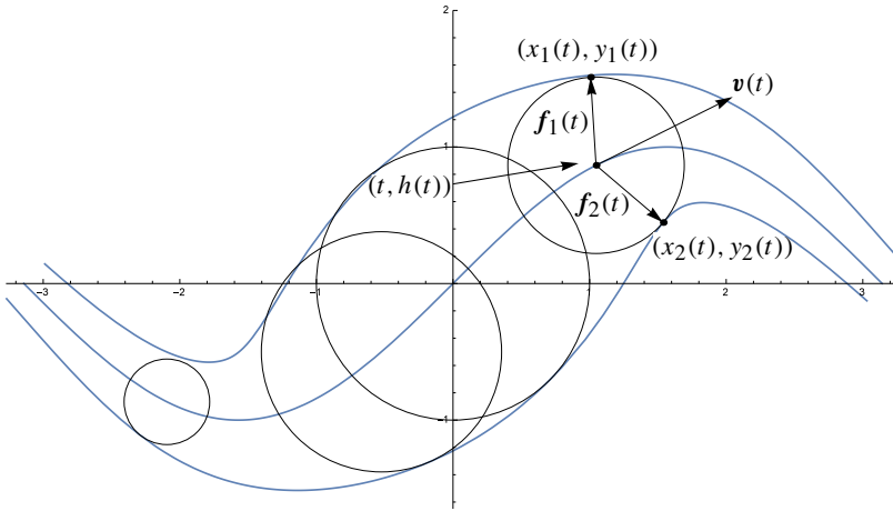
Figure 5. The envelope curves for the circles with centers on the curve y = \sin x and radii given by r(t) = 2/(2+t^2) are shown. The vectors \mathbf{f}_i(t) = (x_i(t) - t, y_i(t) - h(t)) make equal angles with the vector \mathbf{v}(t) = (1, h'(t)) , as asserted by Lemma 3.1.
