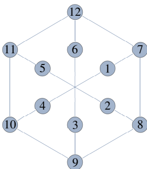
Figure 2. The Petersen graph P(6, 3) .
