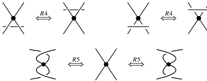
Figure 2. Additional moves for singular links.
