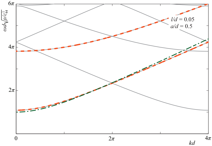
Figure 3. Dispersion curves in the wave number kd -frequency \omega d\sqrt{\rho/c_{44}^1} plane for the antisymmetric modes and l/d = 0.05 and a/d = 0.5 ; solid lines: thick plate with periodic cracks; dotted lines: thick plate with spring boundary conditions; dash-dotted lines: plate equation with spring boundary conditions.
