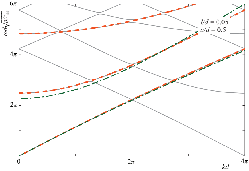
Figure 2. Dispersion curves in the wave number kd -frequency \omega d\sqrt{\rho/c_{44}^1} plane for the symmetric modes and l/d = 0.05 and a/d = 0.5 ; solid lines: thick plate with periodic cracks; dotted lines: thick plate with spring boundary conditions; dash-dotted lines: plate equation with spring boundary conditions.
