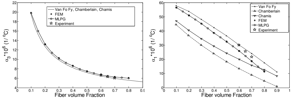
Figure 3. Longitudinal (left) and transverse (right) coefficients of thermal expansion of glass/epoxy composite. “FEM” and “Chamberlain” stand for the values in [Haktan Karadeniz and Kumlutas 2007] and “Experiment” for those in [Sideridis 1994].
