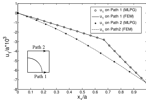
Figure 4. Displacement u_1 on the bottom path ( x_2 = 0 ) and top path ( x_2 = a ) of the RVE in SiC/Ti composite after cooling; \Delta T = -885^\circ\text{C} .
