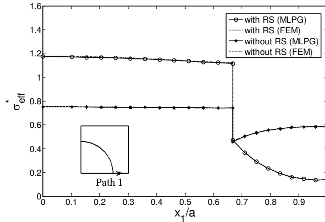
Figure 8. Dimensionless stress \sigma_{\text{eff}}^* on the bottom path for uniaxial tensile load \bar{\sigma}_1 = +0.5Y_m with and without consideration of thermal residual stress.
