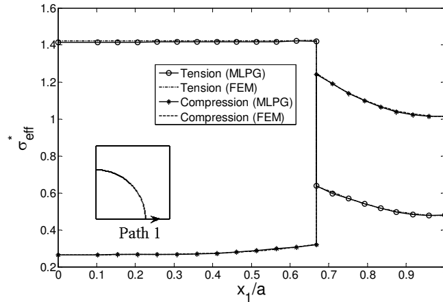
Figure 10. Dimensionless stress \sigma_{eff}^* on the bottom Path 1 of the RVE, biaxial tensile and compressive load \bar{\sigma}_1 = \bar{\sigma}_2 = \pm 0.5Y_m with considering thermal residual stress.
