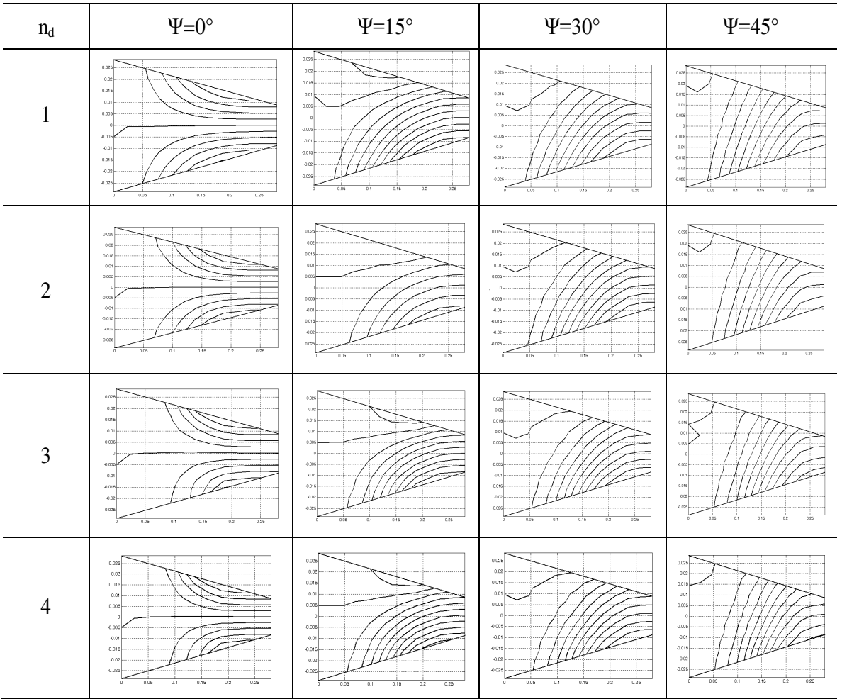
Figure 6. Effect of twist and number of delaminations on mode shapes for NDFB of graphite-epoxy bending-stiff delaminated composite conical shells, considering n = 8 , h = 0.0004 , s/h = 1000 , a/L = 0.33 , d/L = 0.5 , L/s = 0.7 , \theta_0 = 45^\circ , and \theta_v = 20^\circ .
